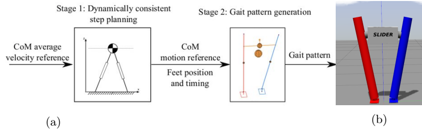
Fig. 4: (a) Overview of the flow of the two-stage pattern generation. The input to the system is an average CoM velocity during individual steps. The first stage uses Linear Inverted Pendulum model to plan the position of feet in sagittal and frontal plane, as well as step time. The second stage based on these information and uses more accurate Multi-Body System model to generate the final gait pattern. (b) the SLIDER simulation in Gazebo.
