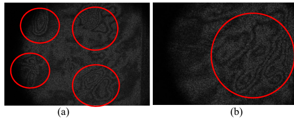
Figure 6. Sample test fringe patterns. Butterfly patterns on the intensity map indicates the delamination on the subsurface of the WTB samples, fringes on SC-45-3 (a), and on SC-45-6 (b)
